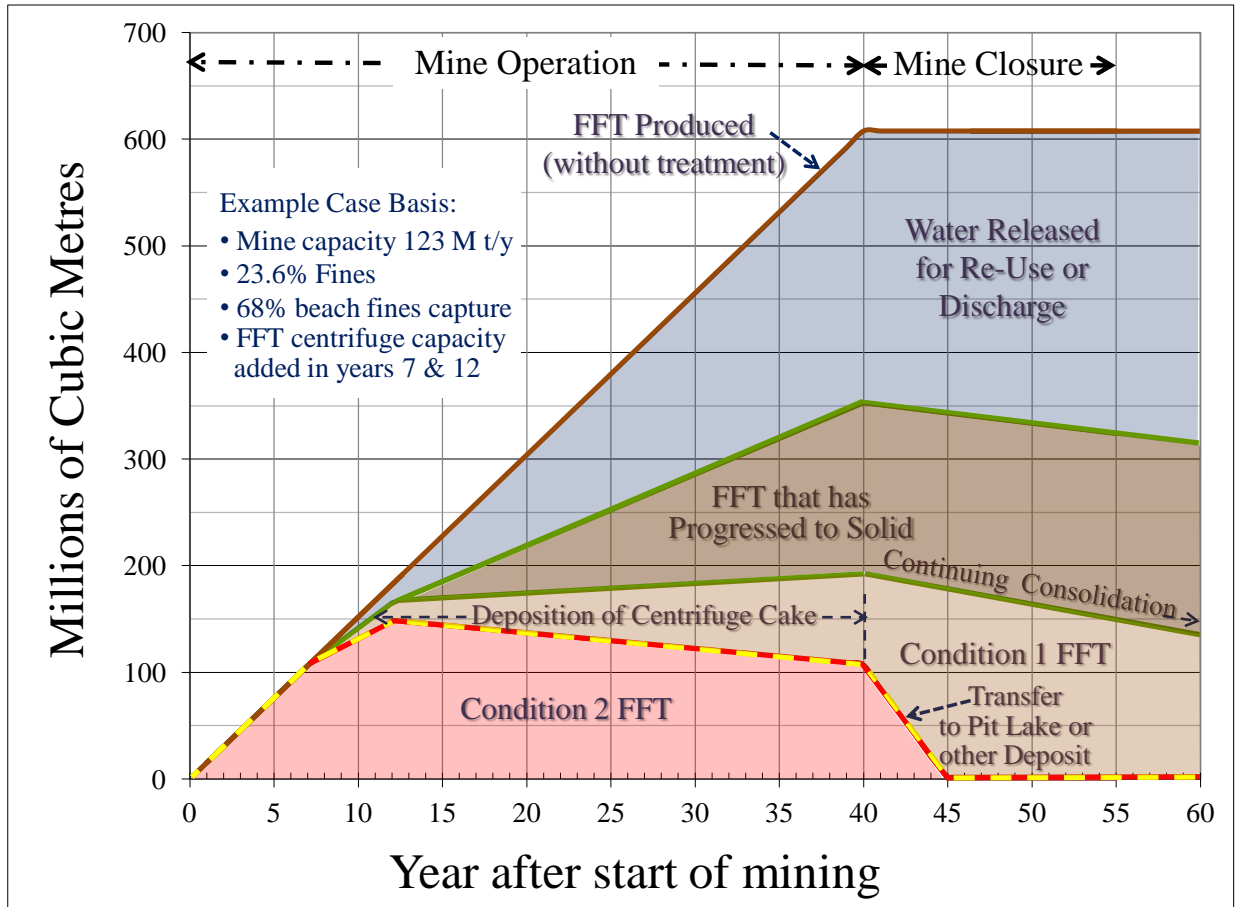
Figure 3-1 Schematic FFT Volume Profiles – (Illustrative Only)
