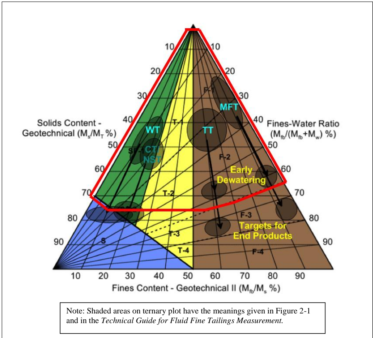
Figure 2-2 Dewatering of Tailings Deposits
