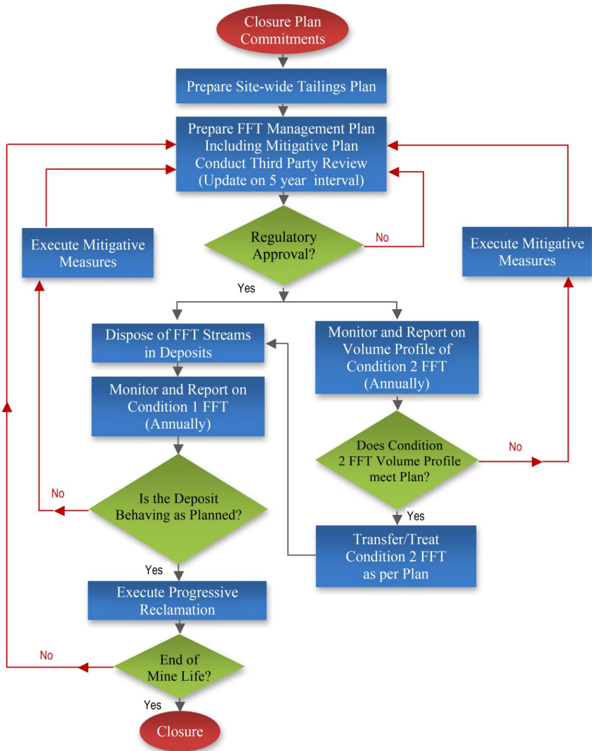
Figure 1-2 Tailings Performance Management Process
