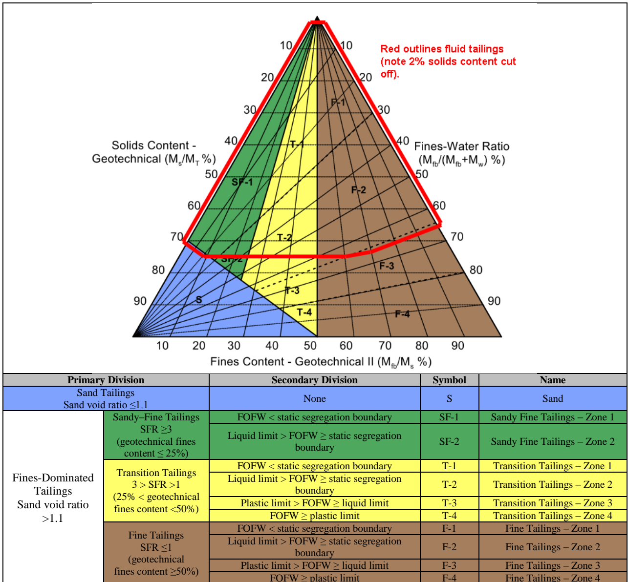
Figure 2-1 Unified Oil Sands Tailings Classification System
